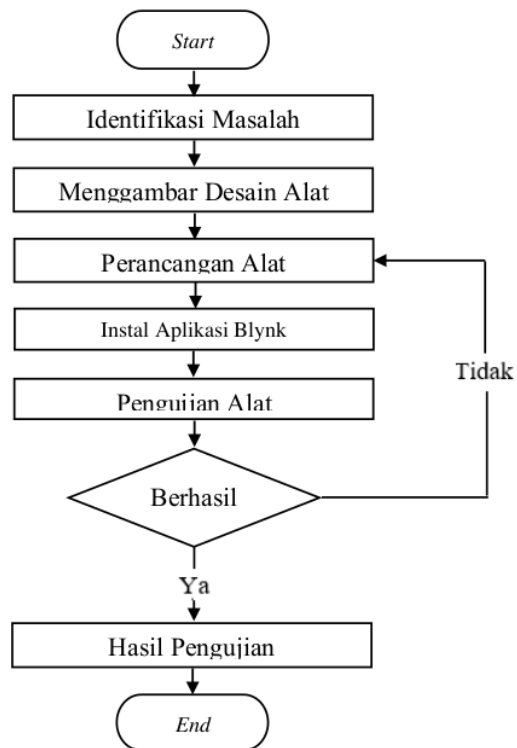
Gambar 1. Flowchart Penelitian
